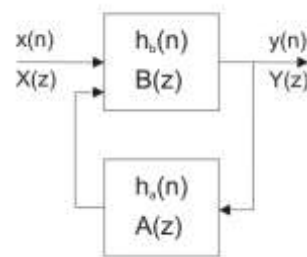
Fig.2 IIR filter block diagram
