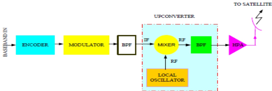
Fig.1. Block Diagram of C-Band Small Satellite Uplink System
