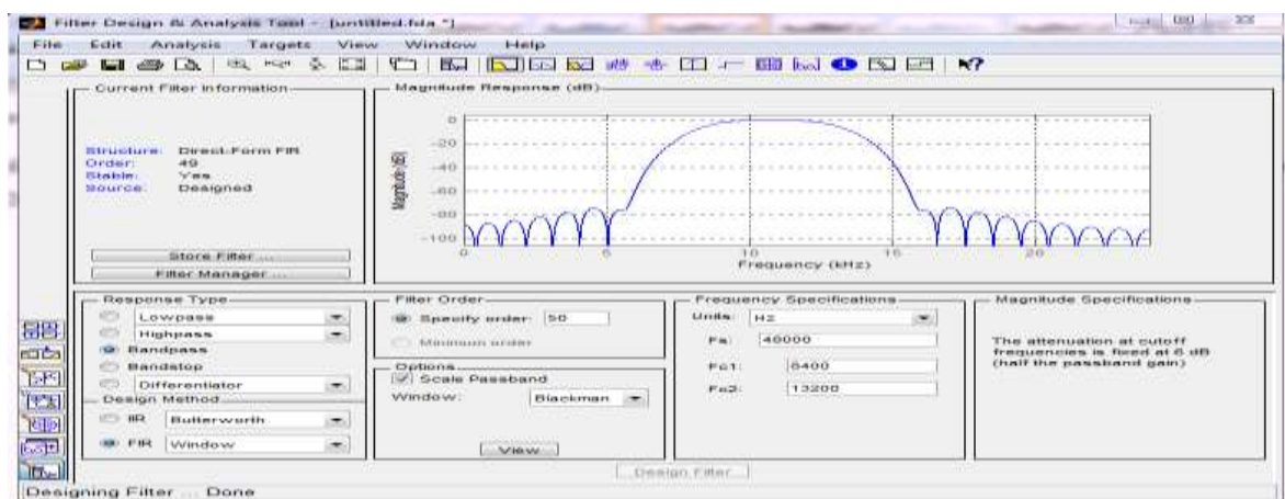
Fig.4: Magnitude response of bandpass filter using blackman window technique
